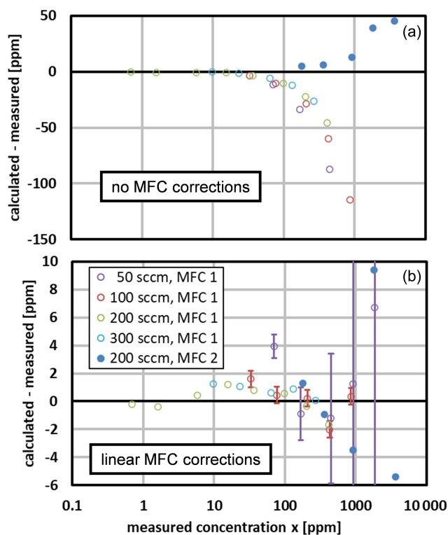
Figure 7. The difference in the calculated and measured mole fractions. The legend denotes the total flow rate and the MFC that supplied gas to the saturator. (a) The initial comparison used the nominal factory calibrations for the MFCs. (b) The final comparison used the linear MFC correction of Eq. (30). Standard uncertainty bars are displayed for two data sets at the larger mole fractions. They correspond approximately to the manufacturer's MFC uncertainties (see Table 6); the uncertainty in the reference hygrometer is negligible here. Note the different vertical scales.
